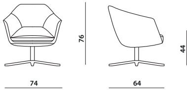
Armchair 4 Spokes
